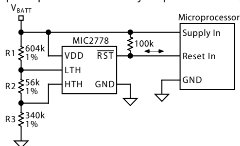
Figure 3. Interfacing to Bidirectional Reset Pin
